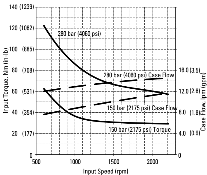
Input Torque and Case Flow Cut-off @ 49°C (120°F)
