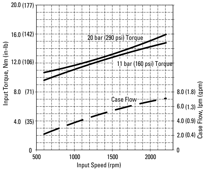
Input Torque and Case Flow Stand-by @ 49°C (120°F)
